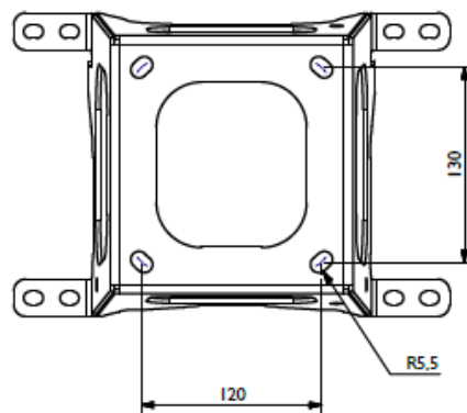
Front view bracket
